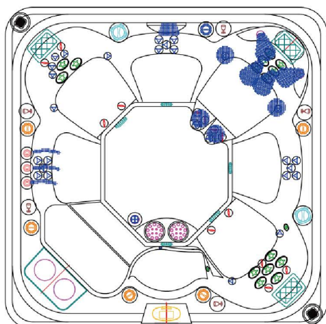
Jet pump 3 16 spa nozzles 1 waterfall 3 fountain
